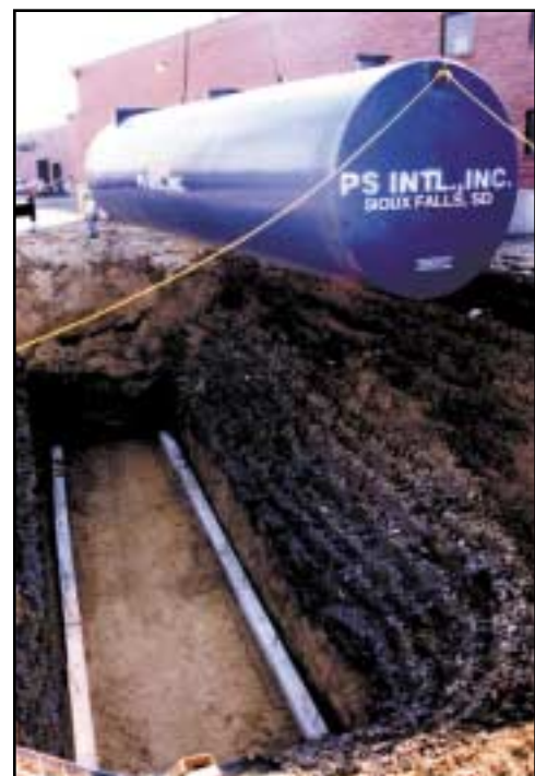
A PS International Model PSC-40,000 double wall separator being installed to treat storm water run-off.
